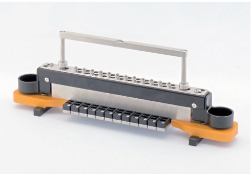
Single Fiber Ferrule (SC, FC) Standard Polishing Processes
