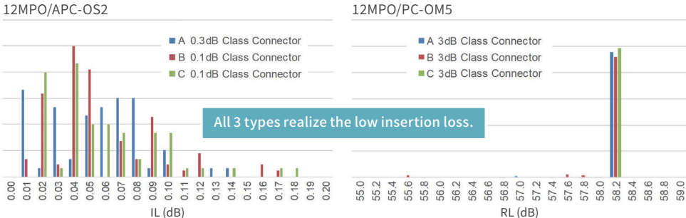
A example of MPO polishing result when ADS-MPO polishing film is used in ATP polishing machine
