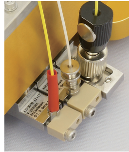
Custom-polishing jigs
