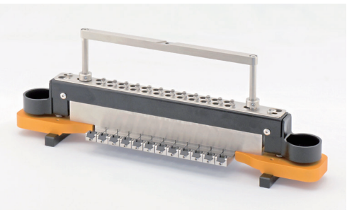
Multi-Fiber ferrule (MT) Polishing Process (reference)
